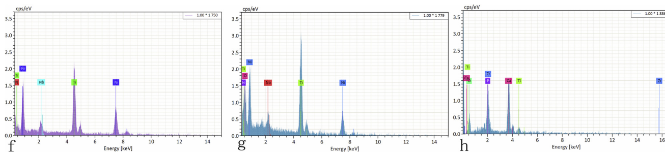
FIGURE 9 – Energy-dispersive spectroscopy of the ProTaper Next X2 file ( f ) unablated area, ( g ) ablated area, and ( h ) dentin fusion area.
