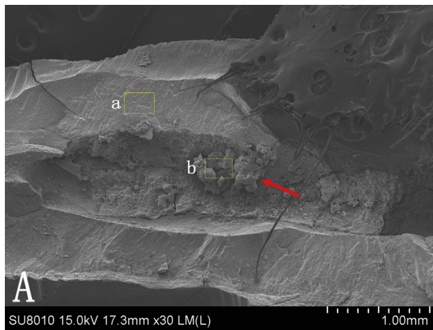
FIGURE 4 – Scanning electron microscopy of the negative control. Dentin fusion ( red arrow ). The energy-dispersive spectroscopic results of areas a and b shown in Figure 7 .
