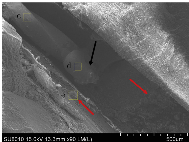
FIGURE 5 – Scanning electron microscopy of the canal with a #15 C-file after ablation. Dentin fusion ( red arrow ) and the file ( black arrow ). The energy-dispersive spectroscopic results of areas c, d, and e shown in Figure 8 .
