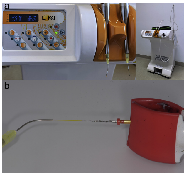
FIGURE 1 – (a) The Lokki laser unit panel and unit and (b) the laser fiber touching the ProTaper Next X2 file at DO.
