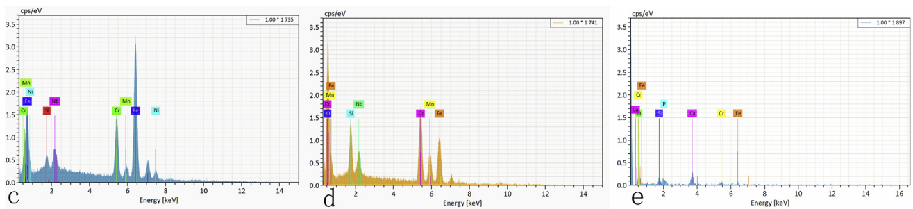
FIGURE 8 – Energy-dispersive spectroscopy of the C-file (c) unablated area, (d) ablated area, and (e) dentin fusion area.
