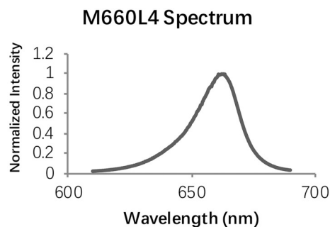
Fig. 1. Spectrum of 660 nm deep red led light source (Data taken from Thorlabs.com). (For interpretation of the references to color in this figure legend, the reader is referred to the web version of this article.)
