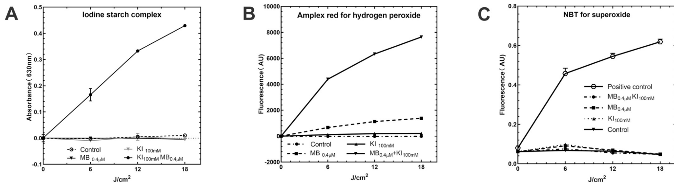
Fig. 8. Mechanistic experiments. A) Production of free iodine measured by starch indicator assay. B) Production of hydrogen peroxide by Amplex red assay. C) Production of superoxide anion by the NBT test. (For interpretation of the references to color in this figure legend, the reader is referred to the web version of this article.)
